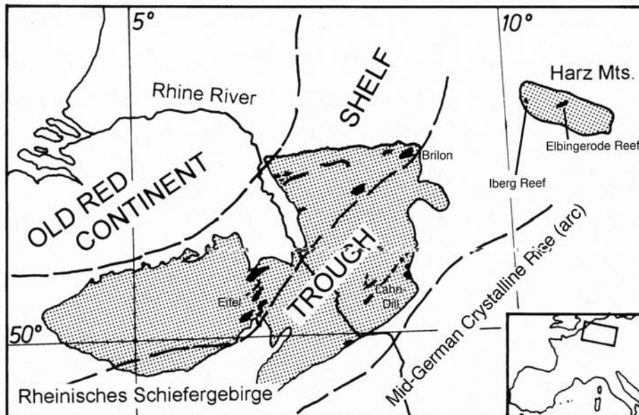
Map of central Europe with Devonian reefs (black) within Palaeozoic outcrops of Rhenisches Schiefergebirge and Harz Mts. (stippled).
